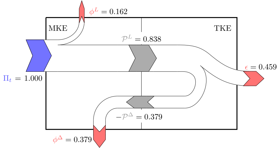
Figure 1: graphical representation of the extended-Reynolds-decomposed energy balance for a Couette flow at h^+ = 101 , where h^+ is the Kármán number.
