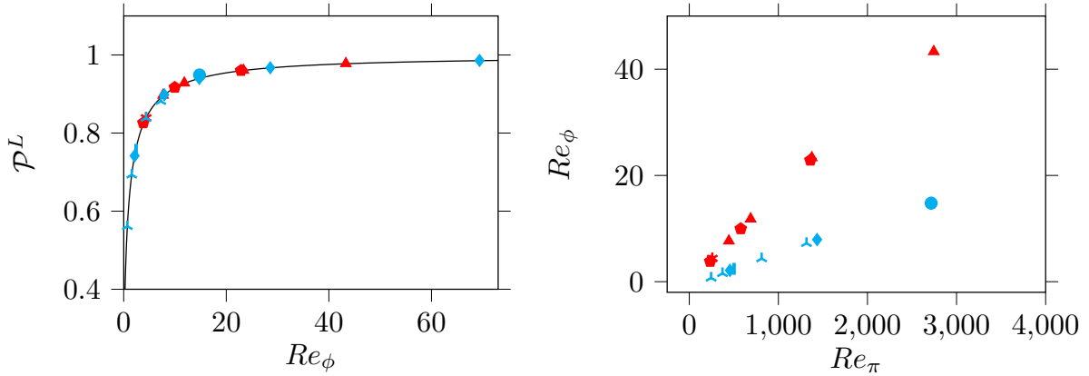
Figure 2: on the left: trend for the turbulent efficiency \mathcal{P}^L against the Reynolds number Re_\phi . Solid line: analytical curve. Numerical data is represented as scatter points; blue is used for Poiseuille, red for Couette. On the right: trend for Re_\phi against Re_\pi ; a constant Re_\pi corresponds to a constant power input.
