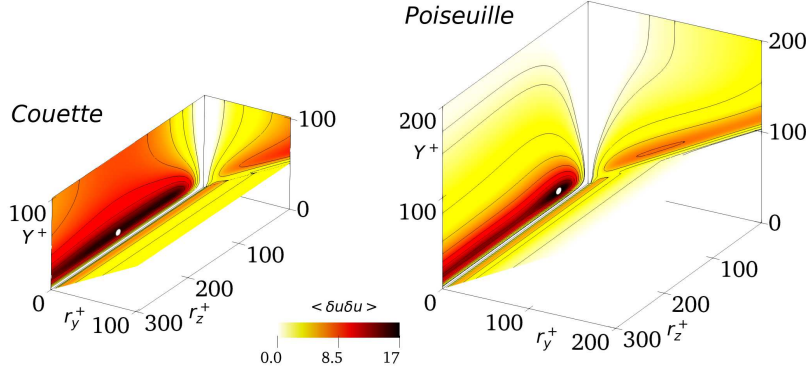
FIGURE 4. Colormap of the structure function \langle \delta u \delta u \rangle in the r_x^+ = 0 space, for Couette (left) and Poiseuille (right). The white marker locates the maximum of the structure function.
