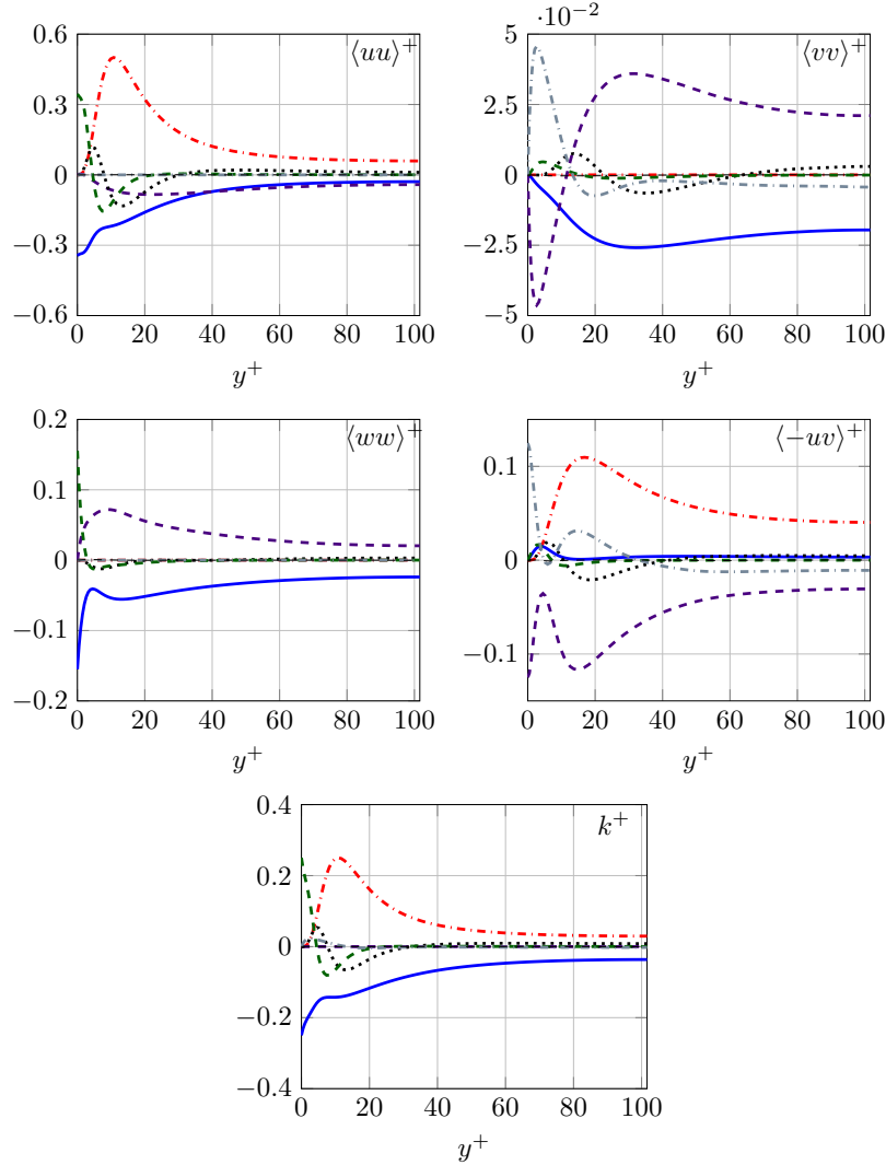
FIGURE 3. Wall-normal profiles of the terms in the budget equation for \langle uu \rangle^+ , \langle vv \rangle^+ , \langle ww \rangle^+ , \langle -uv \rangle^+ and k^+ . The plots feature the turbulent transport ( \cdots ), pressure transport ( -\cdot-\cdot- ), viscous diffusion ( -\cdot-\cdot- ), production ( -\cdot-\cdot- ), pressure strain ( -\cdot-\cdot- ) and pseudo-dissipation ( -\cdot-\cdot- ). The black dashed line plots the imbalance of each equation.
