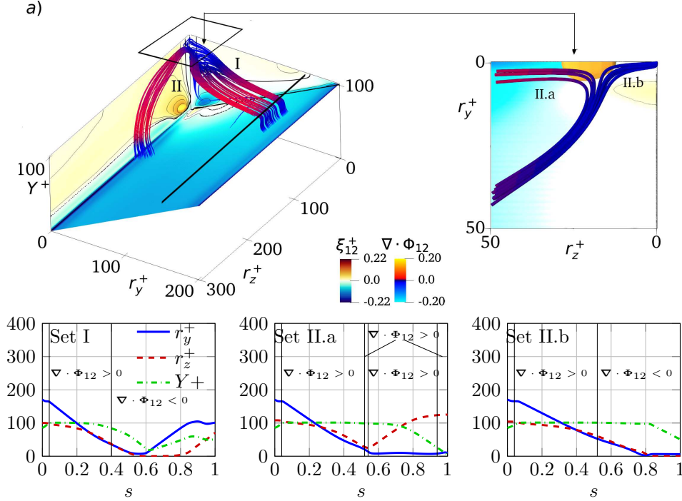
FIGURE 10. Off-diagonal component \langle -\delta u \delta v \rangle . Top: field lines of the vector of the fluxes (\phi_{y,12}, \phi_{z,12}, \psi_{12}) , coloured by the their divergence and grouped in sets I and II. Colour contours of the source term \xi_{12}^+ are shown on the bounding planes, with a black thick line indicating the zero contour level. The black straight line placed at Y^+ = 85 and r_y^+ = 170 indicates all the spanwise separations from which some field lines originate. The yellow isosurface corresponds to \xi_{12}^+ = 0.09 . The top right panel is a zoomed top view of the lines of set II. The evolution of r_y^+ (—), r_z^+ (---) and Y^+ (····) along a representative field line from sets I, II.a and II.b are shown in the lower panels, in which the black vertical lines mark the position where the divergence changes sign along the line.
