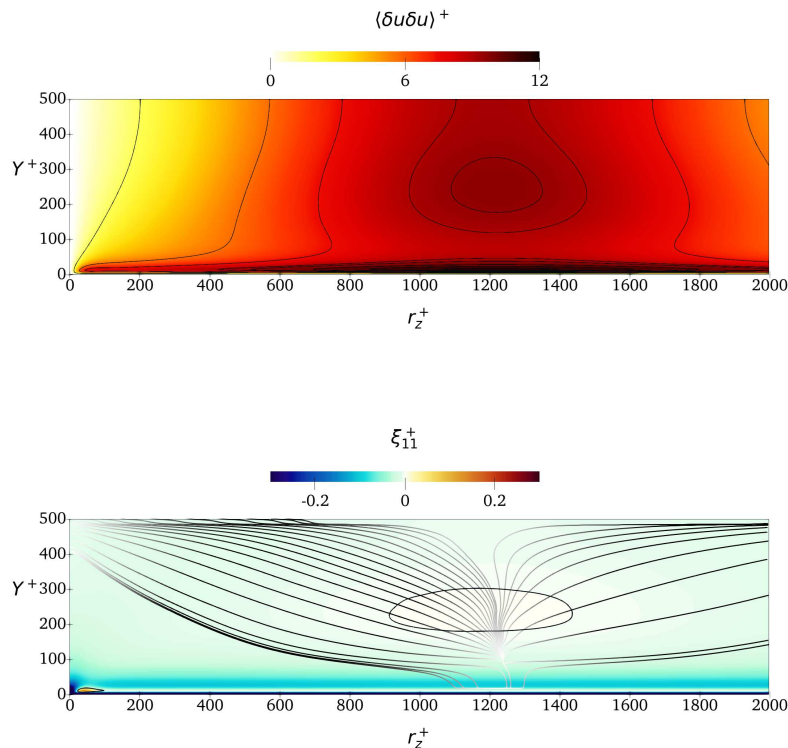
FIGURE 9. Top: \langle \delta u \delta u \rangle at Re_\tau = 500 at r_x = r_y = 0 . Bottom: field lines of the fluxes of \langle \delta u \delta u \rangle coloured with their magnitude, with colormap of the source term shown in the background (black thick lines indicate the zero level).
