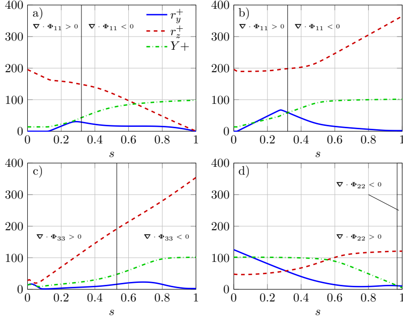
FIGURE 8. Evolution of the values of r_y^+ (—), r_z^+ (---) and Y^+ (-.-) along a representative field line for \langle \delta u \delta u \rangle set I (a) and set II (b); (c) for \langle \delta w \delta w \rangle and (d) for \langle \delta v \delta v \rangle . The dimensionless arch length s is defined as s = 1/s_{max} \int_0^{s_{max}} ds , with ds = \sqrt{dr_y^2 + dr_z^2 + dY^2} . The black vertical lines mark the position where the divergence changes sign along the line.
