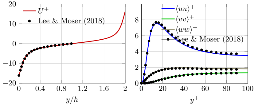
FIGURE 2. Comparison between the present results (color lines) and those by Lee & Moser (2018) (black symbols), obtained at a slightly different Re . Left: mean velocity profile; right: diagonal Reynolds stresses.
