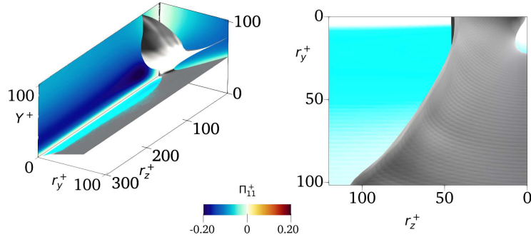
FIGURE 6. Colormap of the pressure-strain term \Pi_{11}^+ for the Couette flow. The grey isosurfaces mark the boundary of non-preferential energy transfer from streamwise fluctuations towards the others. Inner side: \Pi_{22}^+ > \Pi_{33}^+ . Outer side: \Pi_{22}^+ < \Pi_{33}^+ . The right panel is a top view and zoom of the left panel.
