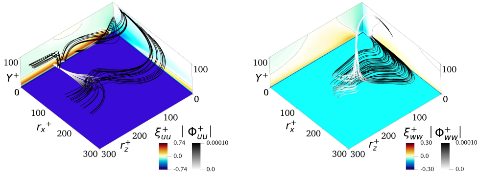
FIGURE 12. Field lines of the vector of the fluxes in the (r_x, r_z, Y) space, for \langle \delta u \delta u \rangle (left) and \langle \delta w \delta w \rangle (right). Colour contours of the corresponding source term are shown on the bounding planes. The flux lines are coloured with the flux magnitude.
