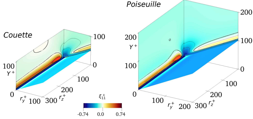
FIGURE 5. Colormap of the source term \xi_{11}^+ for Couette (left) and Poiseuille (right). The colormap on the bounding planes, with the thick line indicating the contour level \xi_{11}^+ = 0 , is plotted together with the isosurface \xi_{11}^+ = 0.55 , which is 75% of the maximum value.
