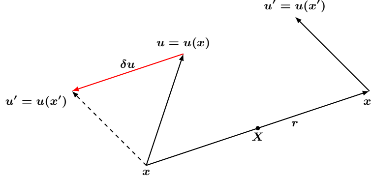
FIGURE 1. Sketch of the quantities involved in the definition of the second-order structure function tensor \langle \delta u_i \delta u_j \rangle . Velocities \mathbf{u} and \mathbf{u}' are evaluated at the points \mathbf{x} and \mathbf{x}' and used to define the increment \delta \mathbf{u} . The midpoint is \mathbf{X} = (\mathbf{x}' + \mathbf{x})/2 , while the separation vector is \mathbf{r} = \mathbf{x}' - \mathbf{x} .
