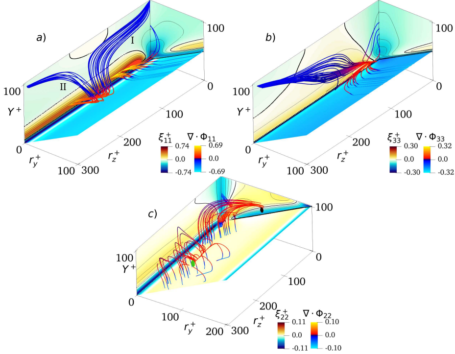
FIGURE 7. Field lines of the vector of the fluxes \Phi = (\phi_y, \phi_z, \psi) coloured by its divergence \nabla \cdot \Phi = \partial\phi_y/\partial r_y + \partial\phi_z/\partial r_z + \partial\psi/\partial Y . Panel (a): \langle \delta u \delta u \rangle ; panel (b): \langle \delta w \delta w \rangle ; panel (c): \langle \delta v \delta v \rangle . Colour contours of the corresponding source term are shown on the bounding planes, with a black thick line indicating the zero level. The isosurfaces correspond to 75% of the source maximum, i.e. \xi_{11}^+ = 0.55 , \xi_{22}^+ = 0.035 , and \xi_{33}^+ = 0.07 . In panel (c), the black dot is the origin of the field lines; the green dot is the singularity point from which other field lines originate.
