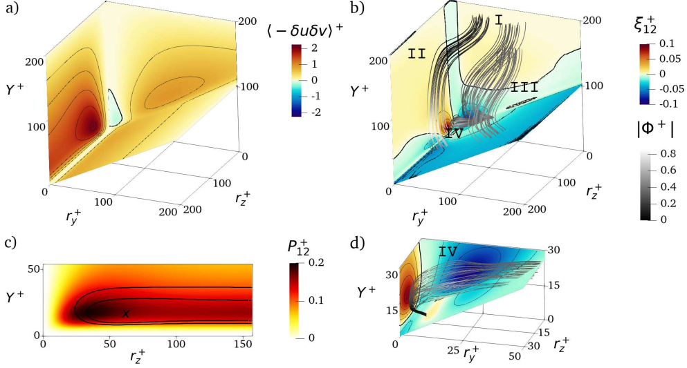
FIGURE 4. Colour plot of \langle -\delta u \delta v \rangle^+ and its budget terms in the 3-dimensional space r_x = 0 . (a) \langle -\delta u \delta v \rangle^+ : contour lines increment by 0.4, with zero indicated by a thick line. (b) Colour plot of \xi_{12}^+ : contour lines increment by 0.02, with zero indicated by a thick line. The gray lines are tangent to the flux vector (\phi_y, \phi_z, \psi) and coloured with its magnitude. A zoom of the region near the origin is shown in panel (d). (c) Colour plot of P_{12}^+ in the r_x = r_y = 0 plane, with isolines for \Pi_{12}^+ demonstrating the different scales involved and the different position of the maximum. The X symbol locates the position of the maximum for \Pi_{12} .
