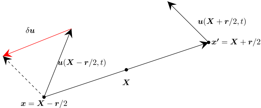
FIGURE 2. Sketch of the quantities involved in the definition of the second-order structure function. \mathbf{x} = \mathbf{X} - \mathbf{r}/2 and \mathbf{x}' = \mathbf{X} + \mathbf{r}/2 are the two points across which the velocity increment \delta\mathbf{u} is computed.
