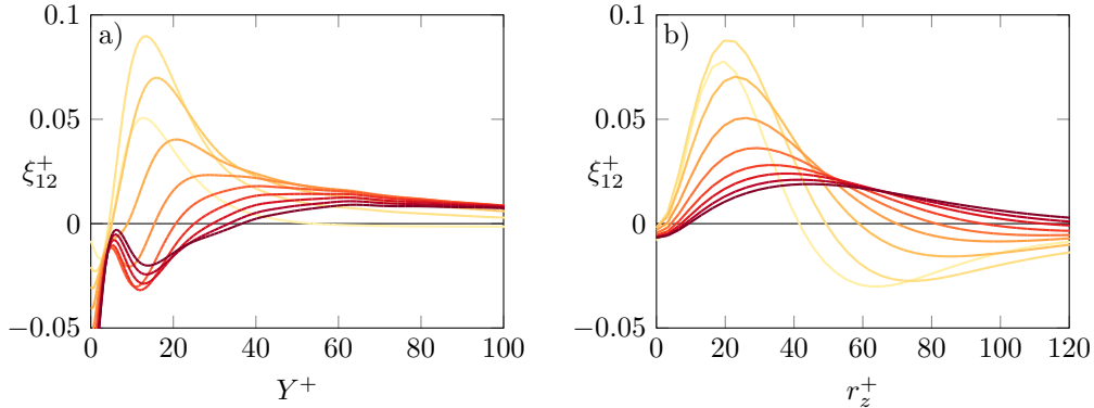
FIGURE 5. Source term \xi_{12} in the r_y = 0 plane. (a) \xi_{12}^+ versus Y^+ for different r_z^+ = (10 : 10 : 100) . (b) \xi_{12}^+ versus r_z^+ for different Y^+ = (10 : 5 : 50) . Line colours encode the value of the parameter, which increases from yellow (light) to red (dark).
