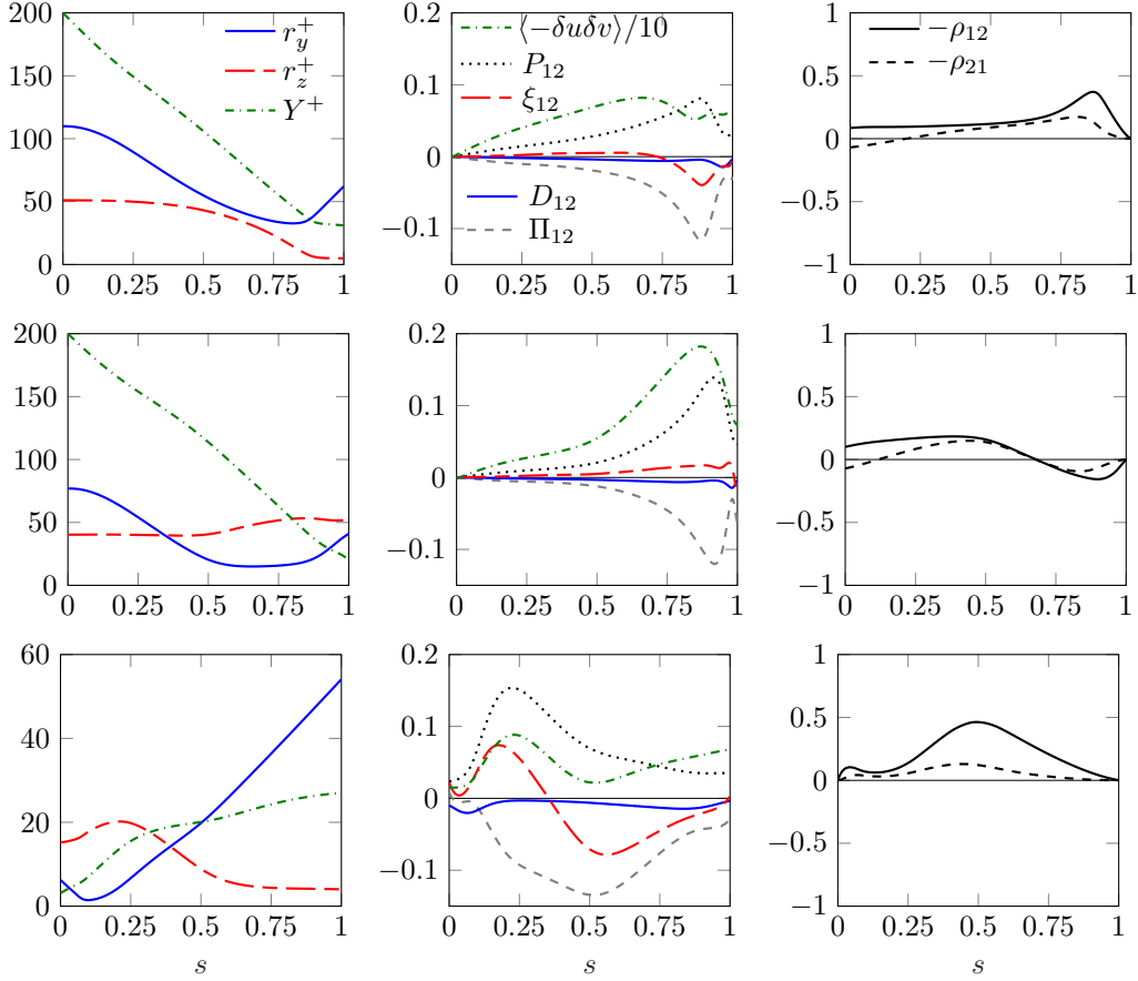
FIGURE 6. Field lines of the flux vector for \langle -\delta u \delta v \rangle . Top: set I; centre: set II; bottom: set IV. Left: evolution of the values of Y (— · — ·), r_y (—), r_z (— —), along a representative field line as a function of its dimensionless arc length s . Centre: values of \langle -\delta u \delta v \rangle / 10 (— · — ·), \xi_{12} (— —), P_{12} (·····), D_{12} (—) and \Pi_{12} (— —) along the line. Right: Evolution of -\rho_{12} (—) and -\rho_{21} (— —) along the line.
