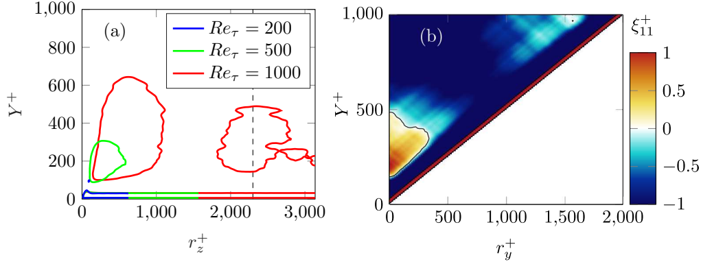
FIGURE 9. (a) Contour \xi_{11} = 0 for Re_\tau = 200, 500 and 1000 in the (r_z, Y) plane at r_x = r_y = 0 . (b) Color map of \xi_{11} at Re_\tau = 1000 in the (r_y, Y) plane for r_x = 0 and r_z^+ = 2300 , i.e. for the plane shown in the left panel (vertical dashed line) which crosses the large-scale \xi_{11} maximum at Re_\tau = 1000 .
