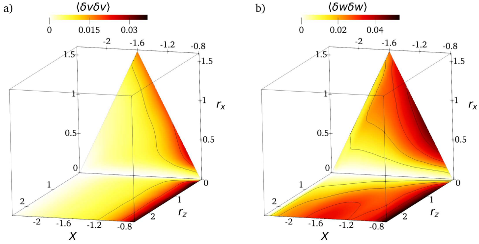
FIGURE 12. \langle \delta v \delta v \rangle (a) and \langle \delta w \delta w \rangle (b) in the (X, r_x, r_z) -space for r_y = 0 and Y = 0.64 . Black contour lines indicate increments by 0.01.
