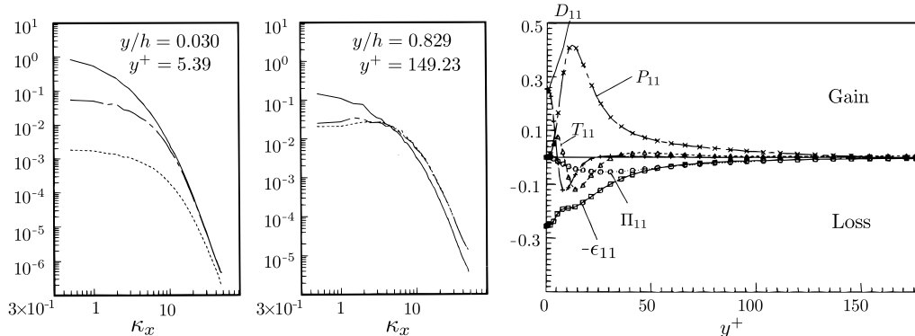
FIGURE 1. Second-order statistics after the seminal DNS of a turbulent channel flow by Kim et al. (1987). Left, adapted from Kim et al. (1987): one-dimensional energy spectra versus streamwise wavenumber \kappa_x , at two wall distances. Continuous, dashed and dotted lines refer to streamwise, spanwise and wall-normal velocity fluctuations. Right, adapted from Mansour et al. (1988): terms in the budget equation for \langle u'_1 u'_1 \rangle , with notation as in the original paper. P_{11} : production; \epsilon_{11} : dissipation; \Pi_{11} : velocity pressure-gradient term; T_{11} : turbulent transport; D_{11} : viscous diffusion.
