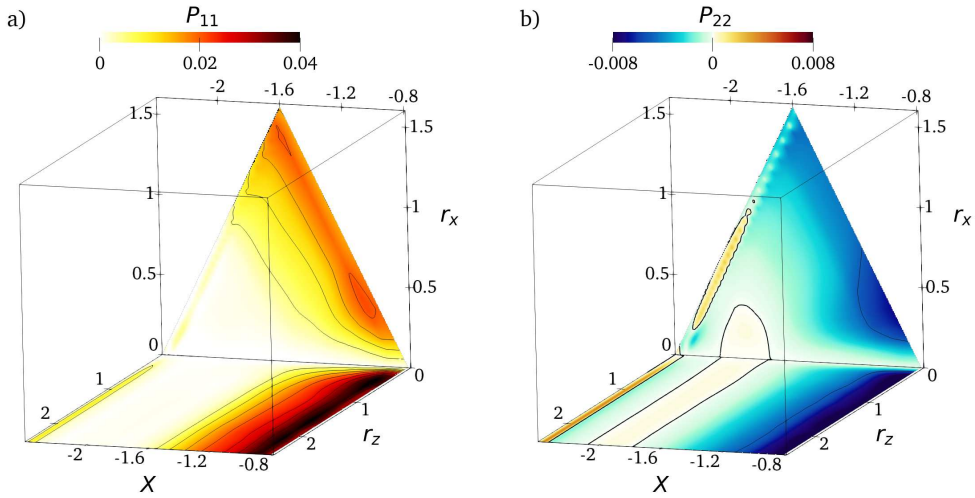
FIGURE 13. Production terms P_{11} (a) and P_{22} (b) in the (X, r_x, r_z) -space for r_y = 0 and Y = 0.64 . Black contour lines indicate increments by 0.005.
