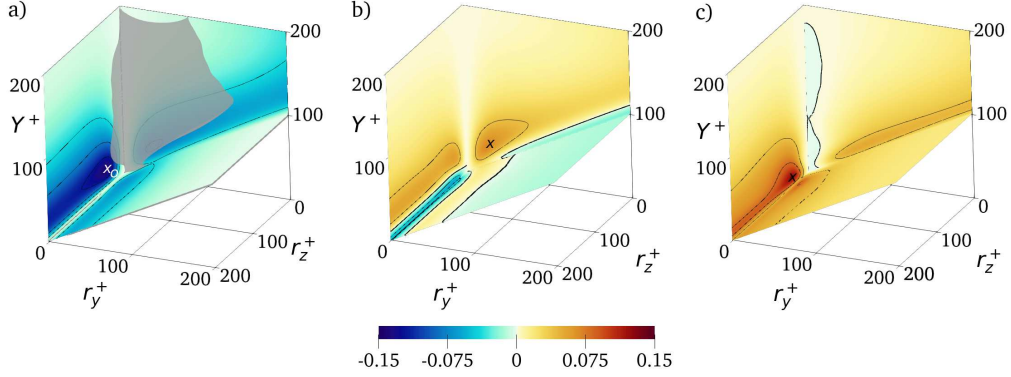
FIGURE 3. Colour plot of: \Pi_{11}^+ (a), \Pi_{22}^+ (b) and \Pi_{33}^+ (c) on the bounding planes r_y^+ = 0 , r_z^+ = 0 and Y^+ = r_y^+/2 . The contour lines increment is 0.04, with level zero indicated by a thick line. The two symbols identify the positions of the maxima of \Pi_{ij} (cross) and P_{ij} (circle). The isosurface in (a) corresponds to \Pi_{22}/\Pi_{11} = -0.5 (or equivalently \Pi_{33}/\Pi_{11} = -0.5 ), with \Pi_{22}/\Pi_{11} < -0.5 for smaller scales.
