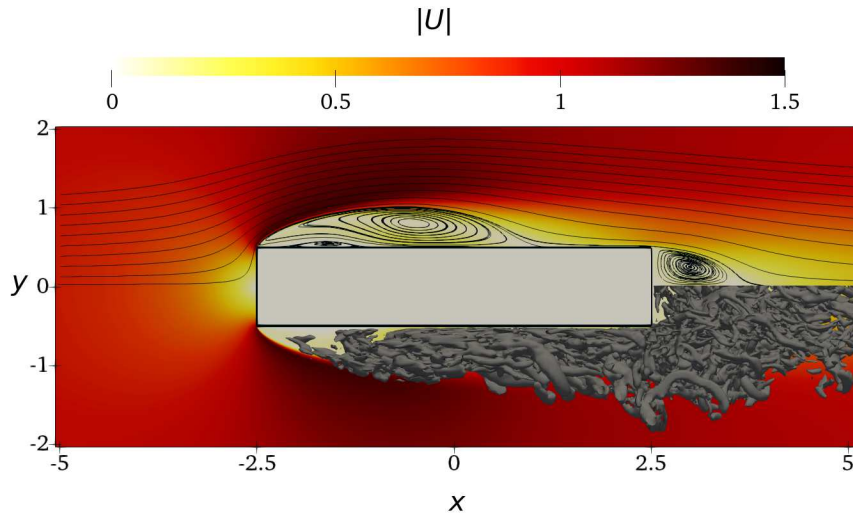
FIGURE 10. Mean and instantaneous flow field around a 5:1 rectangular cylinder at Re = 3000 (flow from left to right; Re is based on free-stream velocity and cylinder height). The color background describes the mean velocity field \mathbf{U}(x, y) = \{U, V, 0\} . In the upper half, mean streamlines show flow detachment at the sharp leading edge, a large recirculation bubble, a smaller secondary bubble and the rear separation in the wake. In the lower half, iso-surfaces for \lambda_2 = -7 visualize instantaneous vortical structures.
