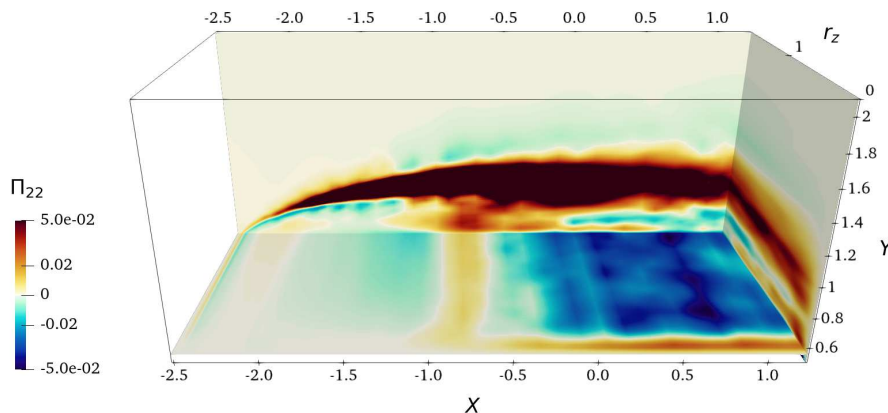
FIGURE 11. Pressure-strain term \Pi_{22} in the (X, Y, r_z) -space for r_x = r_y = 0 . Colour plot are shown on the planes X = 1.2 , Y = 0.56 and r_z = 1.7 .
