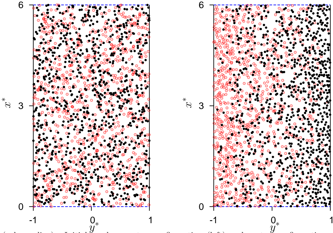
FIG. 1: (color online). Initial random vortex configuration (left) and vortex configuration at t^* = 4.75 \times 10^{-2} (right). Positive and negative vortices are respectively denoted by empty (red) and filled (black) circles.
