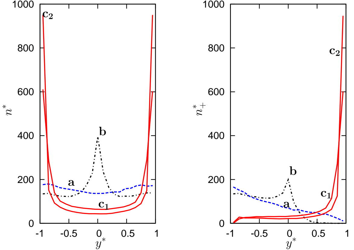
FIG. 3: (color online). Vortex density n^*(y^*) (left) and positive vortex density n_+(y^*) (right) for cases: (a), dashed (blue) line; (b), dot-dashed (black) line; ( c_1 ) and ( c_2 ), solid (red) lines.
