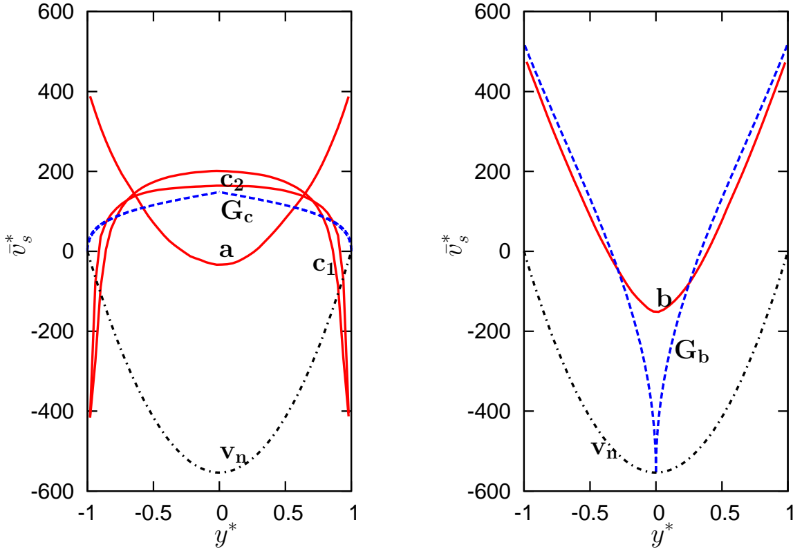
FIG. 2: (color online). Solid (red) line: coarse-grained superfluid velocity \bar{v}_s^*(y^*) ; the labels (a), (c 1 ), (c 2 ) (left) and (b) (right) correspond to the cases discussed in the text. Dashed (blue) line: analytical laminar solution [14] of HBVK equations which applies Geurst’s approach [13] to Cartesian geometry. Curves G_c (left) and G_b (right) correspond respectively to cases (c) and (b) in the text. Dot-dashed (black) line: normal fluid velocity profile (left, right).
