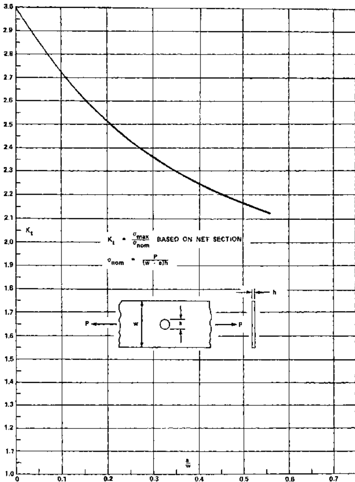
STRESS CONCENTRATION FACTOR, K_t , FOR AXIAL LOADING CASE OF A FINITE-WIDTH PLATE WITH A TRANSVERSE HOLE.
